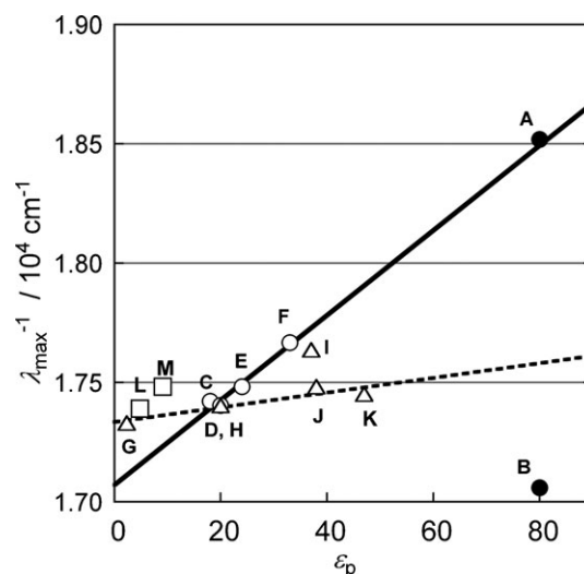
Fig. 9 Variation of \lambda_{\max}^{-1} of PyC8TOV in aqueous solutions (A: c < 0.1 mM, B: c > 2 mM), isopropanol (C), n -propanol (D), ethanol (E), methanol (F), 1,4-dioxane (G), acetone (H), MeCN (I), DMF (J), DMSO (K), \text{CHCl}_3 (L), \text{CH}_2\text{Cl}_2 (M). The solid and dashed lines are obtained by a least-square method for protic polar solvents (C–F), and aprotic polar ones (G–H, J and K), excepting MeCN, 23 respectively.
