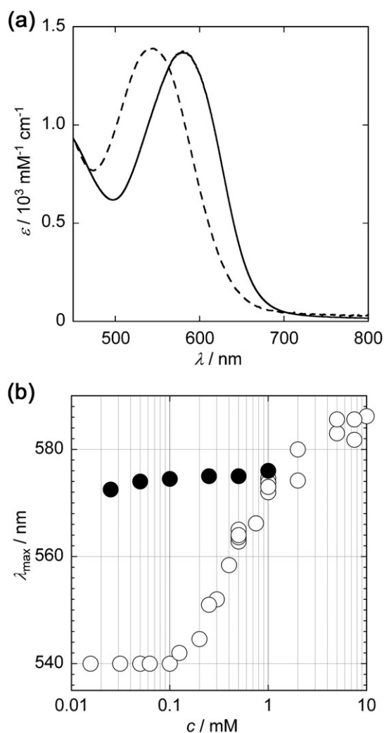
Fig. 3 (a) UV-Vis spectra of PyC8TOV dissolved in water at concentrations of 2.0 (—) and 0.125 (---) mM. (b) Concentration dependence of \lambda_{\max} of PyC8TOV dissolved in water (○) and in \text{CHCl}_3 (●).
