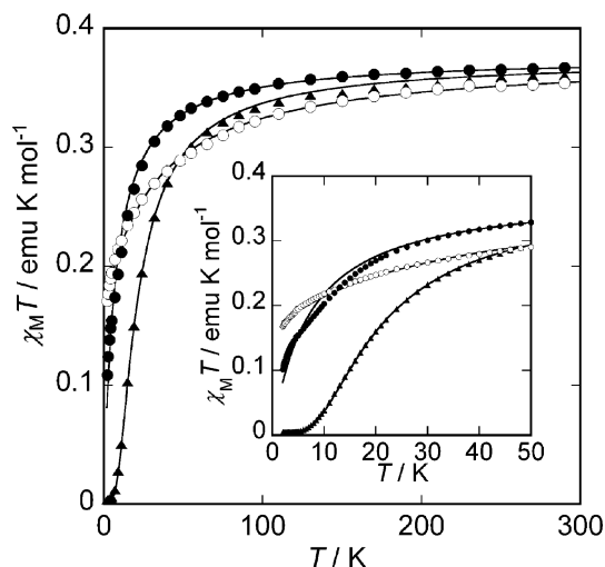
Fig. 2 Temperature dependence of magnetic susceptibilities of microcrystalline PyC8TOV·1.5H 2 O (●), glue-like, anhydrous PyC8TOV (○) and microcrystalline BrC8TOV (▲) as determined by SQUID magnetometer. The solid lines are theoretical fits corresponding to each magnetic structure (see text). Inset: magnified drawing of the low temperature region.
