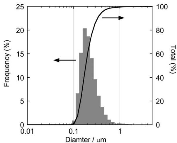
Fig. 4 PyC8TOV aggregate size distribution measurements obtained by dynamic light scattering analysis of a 1 mM aqueous solution of PyC8TOV.
