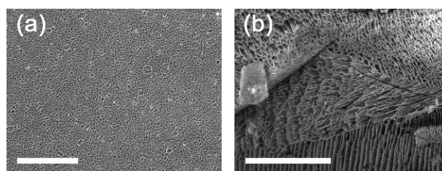
Fig. 5 Phase contrast microscopic image (a) and cryo-SEM image (b) of a 20 mM aqueous solution of PyC8TOV. Scale bars: 100 \mu\text{m} .
